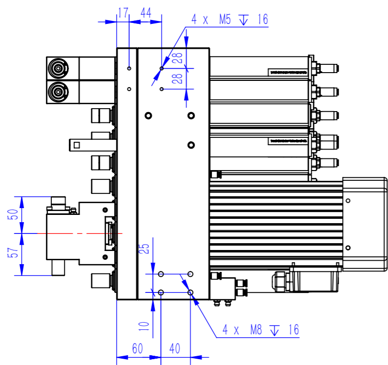
View A
