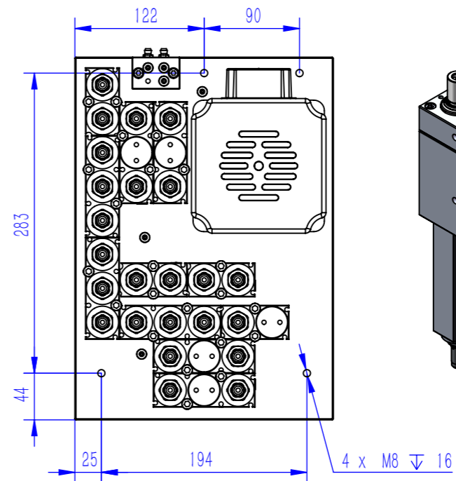
View B
