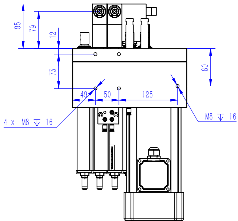
View A
